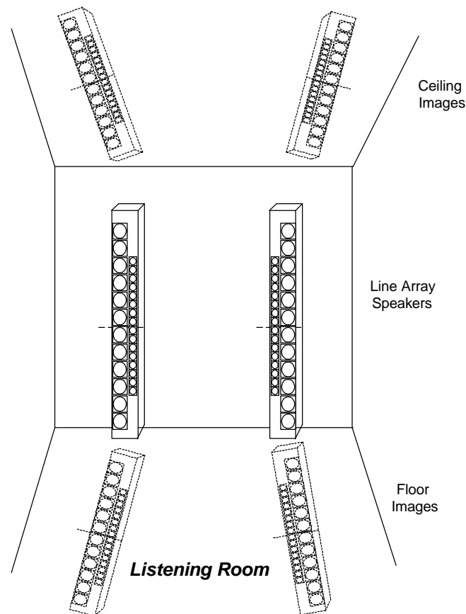
Figure 6. Low Frequency Floor and Ceiling Mirror Image Reflections
